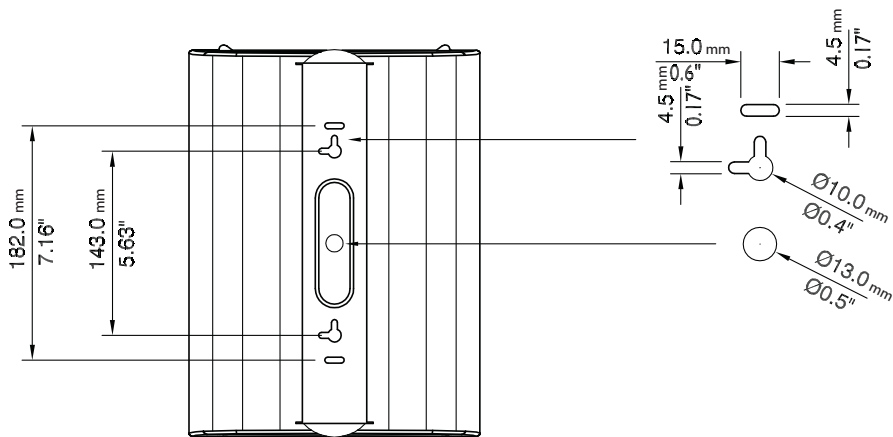
Rear View
